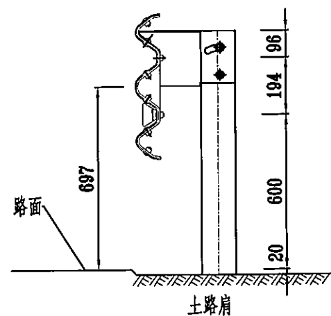
De-Rby (Rbw)-At1轮廓标安装立面图1 1:20
